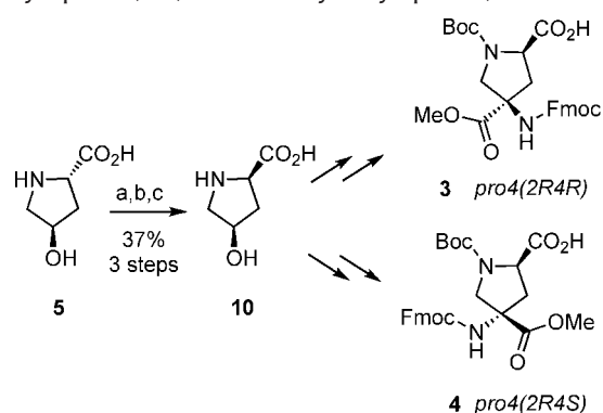
SCHEME 2. The Synthesis of the pro4(2R4R) ( 3 ) and pro4(2R4S) ( 4 ) Monomers Follows the Route Shown in Scheme 1 Substituting cis -4-Hydroxy-D-proline, 10 , for trans -4-hydroxy-L-proline, 5 a
