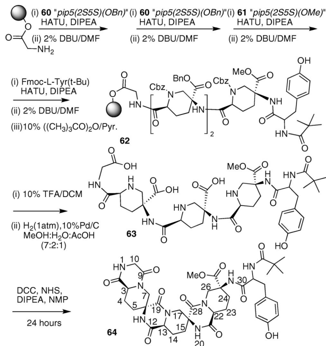
SCHEME 8. Synthesis and Chemical Structure of Oligomer 64
