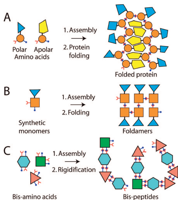
FIGURE 1. A comparison of bis-peptides to other approaches to forming structured macromolecules: (A) In proteins, widely separated apolar amino acids fold together to avoid water, and intrasidic hydrogen bonds help to stabilize the folded structure. (B) Foldamers are synthetic oligomers that fold into well-defined secondary structures due to the conformational preferences of their monomers, local inter-residue hydrogen bonds, and solvophobic tendencies of their monomers. (C) Bis-peptides are synthetic oligomers assembled from cyclic, stereochemically pure monomers coupled through pairs of amide bonds to form rigid spiro ladder oligomers with predefined and programmable three-dimensional structures.
